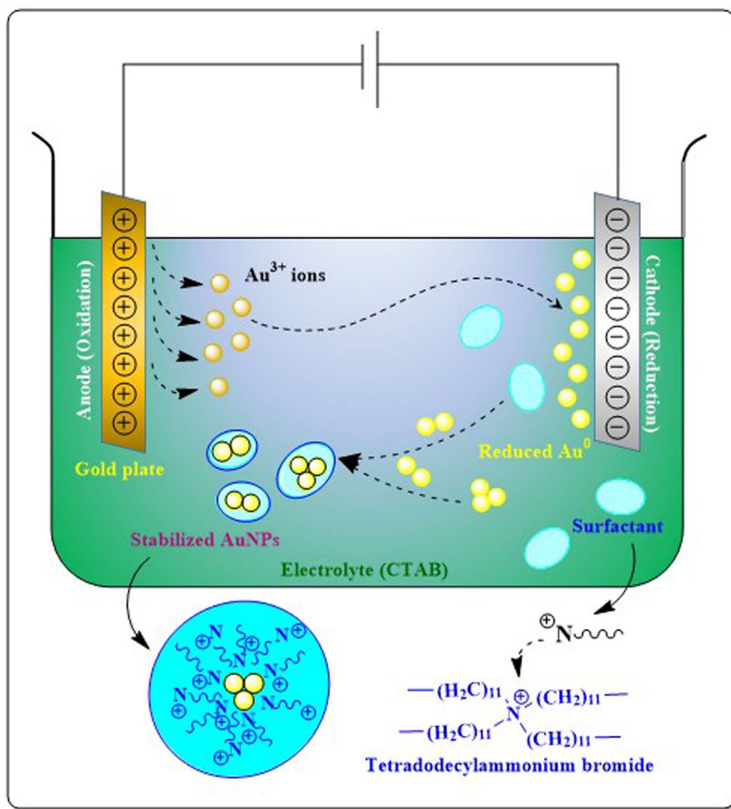
Fig. 6 Electrochemical method for AuNP synthesis. During electrolysis, a gold plate used as an anode generates Au 3+ ions, which are attracted towards the oppositely charged cathode and reduction takes place. After reduction, the random attachment of Au 0 ions forms nanogold stabilized by surfactants like TAAB (in the figure tetradodecylammonium bromide).
