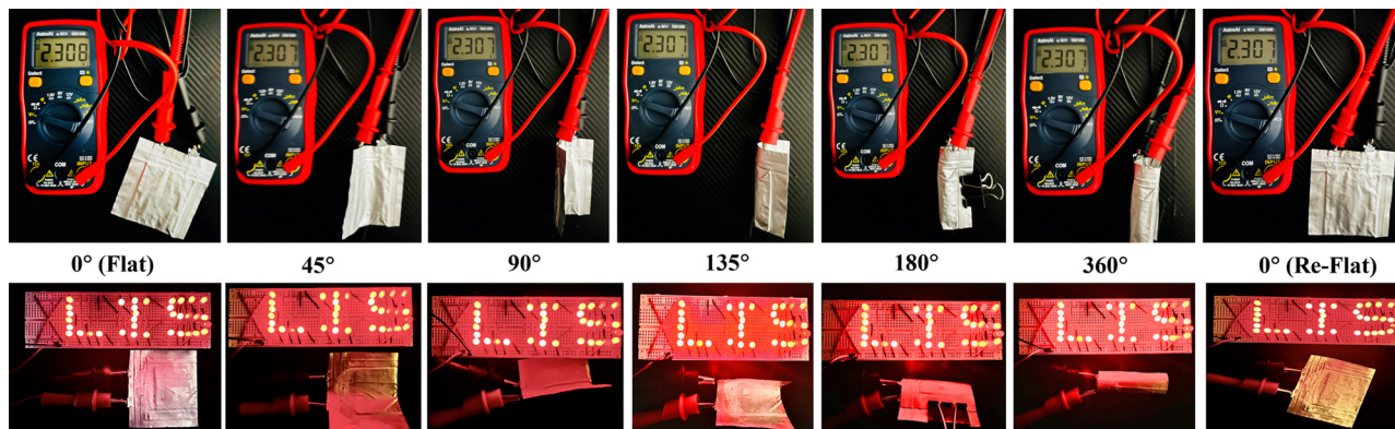
Fig. 6 Upper row: digital pictures of the OCV for the pouch cell consisting of the g\text{-C}_3\text{N}_4\text{-Mx/S} cathode at different folding angles. Bottom row: pictures of LEDs lightening up by a pouch cell at different folding angles demonstrating the excellent flexible feature of the developed pouch cell.
