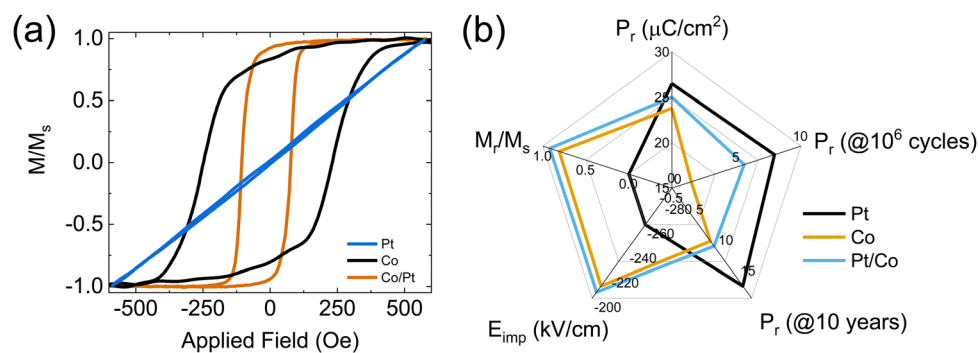
Fig. 4 (a) MOKE signal normalized to its value at 550 Oe when using Pt, Co and Pt/Co top electrodes. (b) Summary of ferroelectric and magnetic characteristic parameters of samples with Pt, Co and Pt/Co top electrodes.
