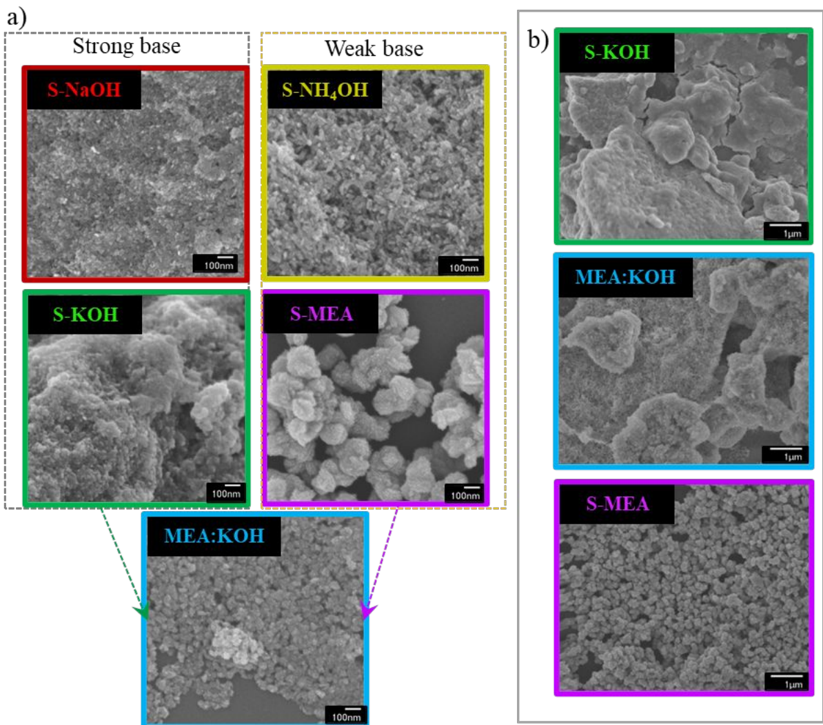
Figure 4. SEM images of the S-NH 4 OH, S-NaOH, S-KOH, S-MEA, and MEA/KOH catalysts in 50 kx magnification (a) and comparison of the S-KOH, S-MEA, and MEA/KOH catalysts in lower magnification of 10 kx.
