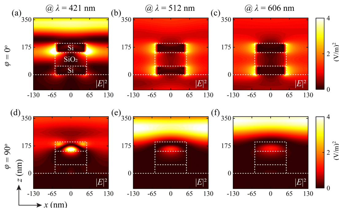
Fig. 3 The xz-view of the spatial electric field ( |E|^2 ) distributions at the wavelengths of 421, 512, and 606 nm for (a)–(c) \varphi = 0^\circ and (d)–(f) \varphi = 90^\circ . The white dotted lines denote the proposed dielectric metasurface structure.
