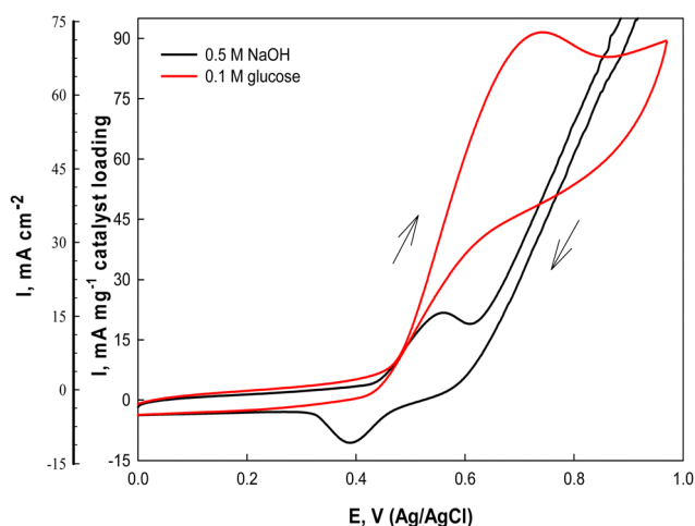
Fig. 7 Cyclic voltammograms of the Ni(II)-SB/C electrode in 0.5 M NaOH and in the presence of 0.1 M glucose at 0.02 \text{ V s}^{-1} .
