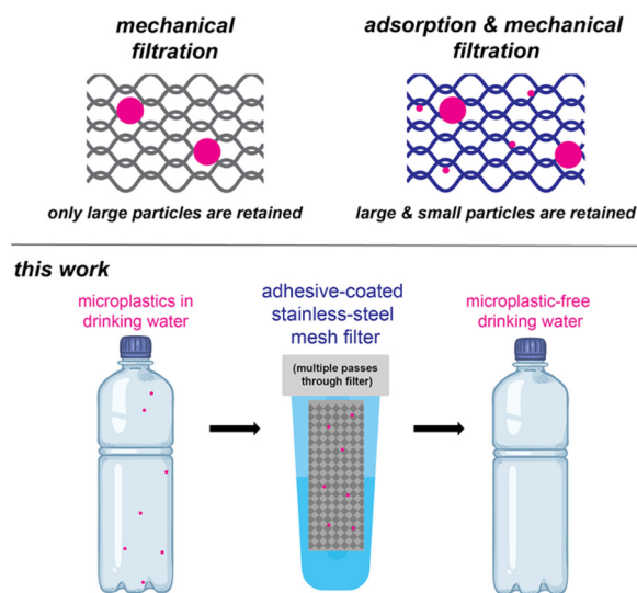
Scheme 1 Filtering mechanisms (top) and an adhesive-coated stainless-steel filter for removing microplastics from drinking water (bottom).
