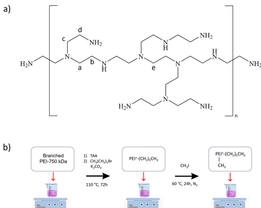
Fig. 1 (a) Chemical structure of branched PEI (750 kDa); (b) schematic route to alkylated PEIs synthesis.
