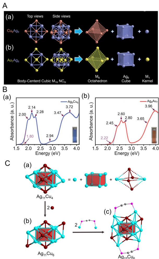
Fig. 13 (A) Anatomy of (a) [\text{Ag}_9\text{Cu}_6(\text{C}\equiv\text{C}'\text{Bu})_{12}]^+ and (b) [\text{Ag}_7\text{Au}_3(\text{C}\equiv\text{C}'\text{Bu})_{12}]^+ . Color legend: Au, yellow; Ag, purple; Cu, orange. (B) Experimental absorbance spectra plotted in the energy axis of (a) [\text{Ag}_9\text{Cu}_6(\text{C}\equiv\text{C}'\text{Bu})_{12}]^+ and (b) [\text{Ag}_7\text{Au}_3(\text{C}\equiv\text{C}'\text{Bu})_{12}]^+ . (C) Structure analysis of the [\text{Ag}_{15}\text{Cu}_6(\text{C}\equiv\text{CPh}(\text{CF}_3)_2)_{18}(\text{DPPE})_2]^- . (a) Structure anatomy of the \text{Ag}_{11}\text{Cu}_4 metal core. (b) Capping of two opposite \text{Ag}_3 faces of the \text{Ag}_{11}\text{Cu}_4 core forms the structure of \text{Ag}_{11}\text{Cu}_6 . (c) Stabilization of the \text{Ag}_{11}\text{Cu}_6 metal framework by two \text{Ag}_2\text{DPPE} motifs forms the structure of [\text{Ag}_{15}\text{Cu}_6(\text{C}\equiv\text{CPh}(\text{CF}_3)_2)_{18}(\text{DPPE})_2]^- . Color legend: turquoise, Ag; dark red, Cu; pink, P; gray, C. (A) and (B) are reproduced with permission from ref. 244. Copyright 2021 Royal Society of Chemistry. (C) is reproduced with permission from ref. 263. Copyright 2022 American Chemical Society.
