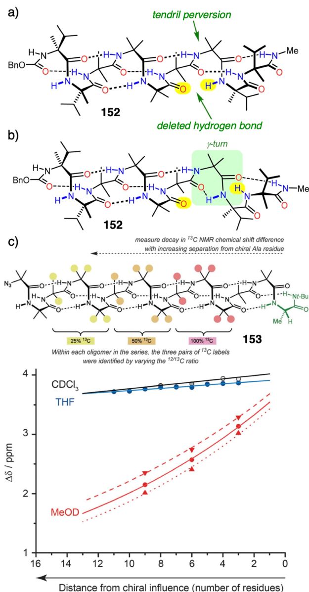
Fig. 74 (a) Tendrils or perversions and (b) \gamma -turn in AIB foldamer 152 . (c) Chemical shift differences ( \Delta\delta ) measured in a series of three 'frame-shifted' oligomers, each containing three pairs of abundance-labelled (100%, 50% or 25%) ^{13}\text{C} labels. Screw-sense preference exhibited by Aib oligomer 153 decays as a terminal chiral influence becomes more distant. Reproduced from ref. 358 with permission from the Royal Society of Chemistry, copyright 2016.
