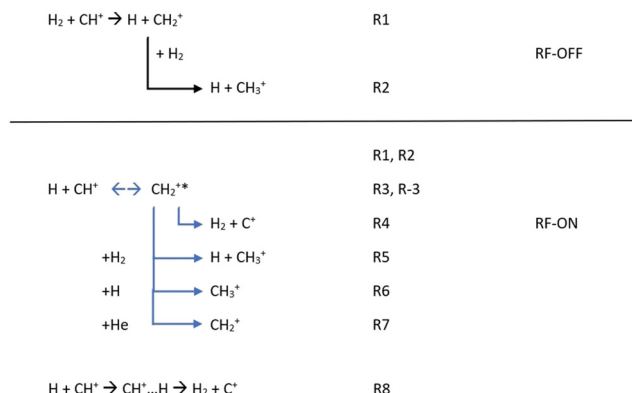
Fig. 3 Chemical reactions possibly occurring in the experimental setup with the RF discharge set to OFF and ON.
