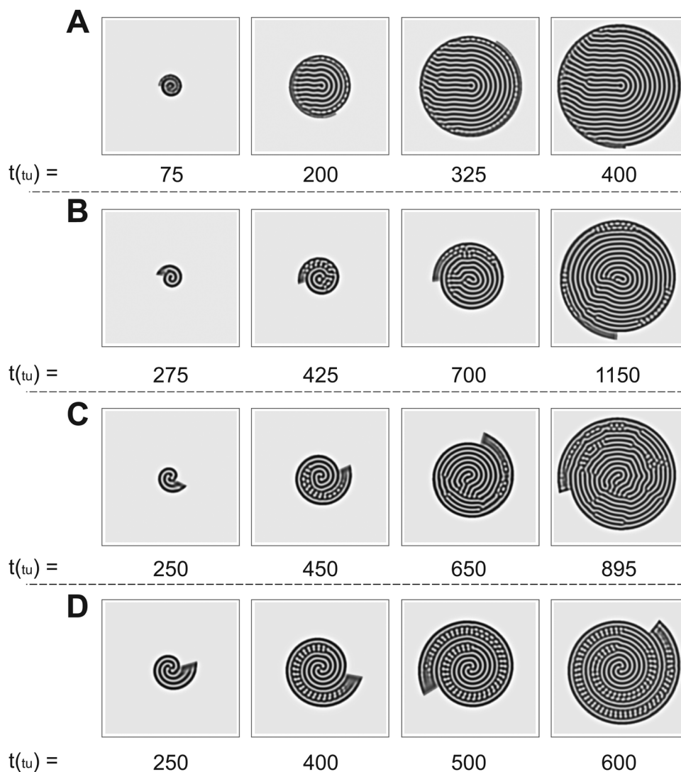
Fig. 5 Time evolution of transitional structures obtained in numerical simulations for (A) n = 0.5 ( \dot{r}_T = 0.242 \text{ su/tu} , \dot{\theta}_T = 24.0^\circ/\text{tu} ), (B) n = 1.55 ( \dot{r}_T = 8.05 \times 10^{-2} \text{ su/tu} , \dot{\theta}_T = 2.58^\circ/\text{tu} ), (C) n = 2.6 ( \dot{r}_T = 0.107 \text{ su/tu} , \dot{\theta}_T = 2.05^\circ/\text{tu} ), and (D) n = 3.6 ( \dot{r}_T = 0.161 \text{ su/tu} , \dot{\theta}_T = 2.22^\circ/\text{tu} ) in a 200 \text{ su} \times 200 \text{ su} domain.
