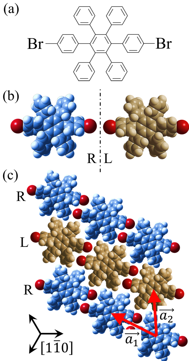
Fig. 1 (a) Chemical structure of Br 2 -HPB. (b) Space-filling models of the molecular chiralities. The enantiomeric R- and L-types are defined by the CW and CCW rotations of the outer phenyl rings with respect to the central benzene ring. The blue and brown coloured models represent the R- and L-types chiralities, respectively. (c) Self-assembled structure of Br 2 -HPB molecules described by the unit cell vectors \vec{a}_1 and \vec{a}_2 . The lattice parameters have been obtained as |\vec{a}_1| = 14.3 \pm 0.3 \text{ \AA} , |\vec{a}_2| = 12.8 \pm 0.3 \text{ \AA} , the included angles 57.2 \pm 3.1^\circ , and the molecular orientation defined by opposite bromine atoms is rotated by about 11^\circ from the [1\bar{1}0] direction of the underlying Au(111) surface. 26 The molecular chiralities tend to be ordered in R- or L-homochiral arrangements in the \vec{a}_1 direction with a 62% probability, and in RL-heterochiral arrangement in the \vec{a}_2 with a 81% probability.
