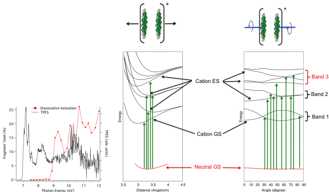
Fig. 8 Left: photoionization (black) and photoionization + dissociation (red) spectra for Py 2 recorded at SOLEIL synchrotron apparatus. Right: computed electronic ground states of Py 2 and Py 2 + and first electronic excited states of Py 2 + according to dissociative breathing mode (left) and non-dissociative twist mode (right). Adapted from ref. 222 with permission from the PCCP Owner Societies. Copyright 2023.
