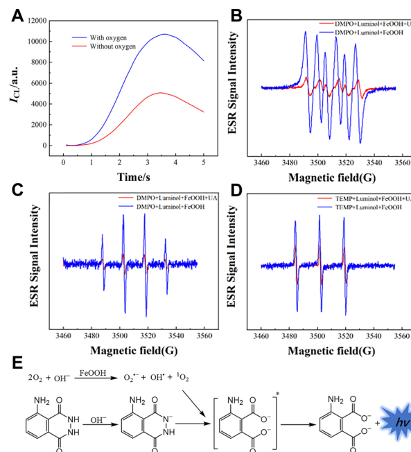
Fig. 12 (A) CL kinetic curves of the luminol/FeOOH system in the absence and presence of oxygen. ESR spectra of adducts. (B) DMPO-O 2 * (C) DMPO-OH* and (D) TEMP-O 2 * in the luminol/FeOOH CL system. (E) Mechanism of the luminol/FeOOH CL system. [Luminol]: 100 μM; [FeOOH]: 25 μg mL -1 ; [UA]: 5 μM; [pH]: 10.0. Reprinted with permission from ref. 63, Copyright 2023 American Chemical Society.
