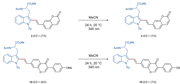
Scheme 3 Isomerization studies.
