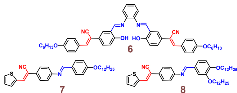
Fig. 12: Chemical structures of probes 6-8.
