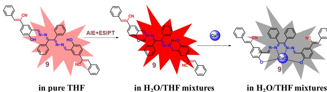
Fig. 13: Chemical structure of probe 9 and the proposed mechanism of probe 9 with Cu 2+ ions.
