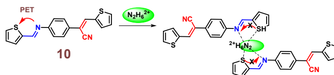
Fig. 15: Proposed sensing mechanism of 10 with \text{N}_2\text{H}_6^{2+} ions
