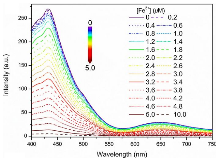
Fig. 22: Emission spectra of probe 16 (10 \mu\text{M} ) with various concentration of \text{Fe}^{3+} ions in THF/water mixtures ( f_w = 90\% , \text{pH}=7.4 , \lambda_{\text{ex}}=380\text{ nm} ). Reproduced with permission from ref. 61. Copyright 2024 elsevier.
