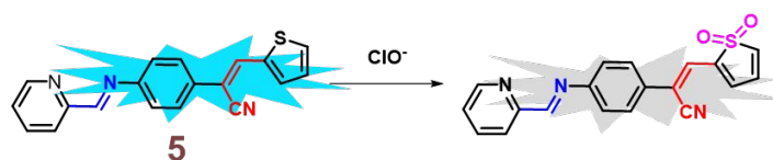
Fig. 8: Proposed sensing mechanism of 5 with \text{ClO}^- ions
