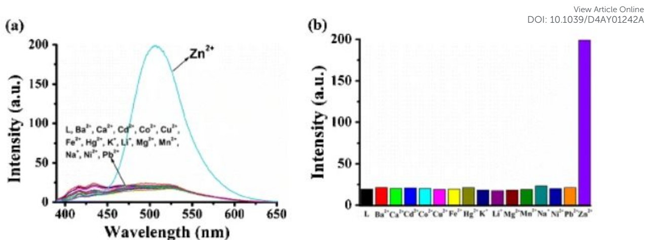
Fig. 4: a) Emission spectra of probe 2 alone and with different metal ions. (b) Fluorescent intensity of 2 at 509 nm with different metal ions. Reproduced with permission from ref. 48. Copyright 2014 Springer.
