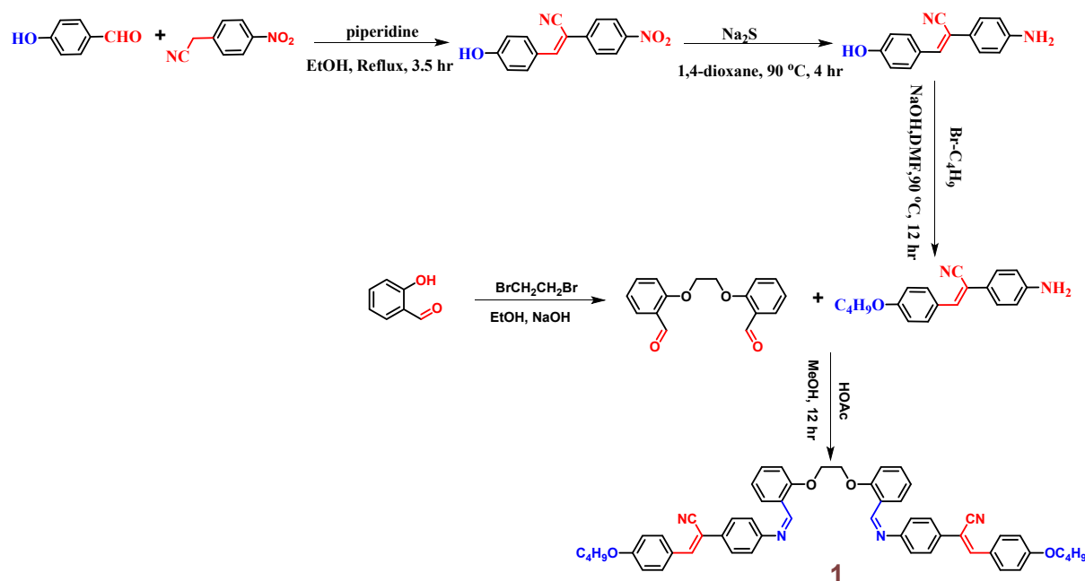
Scheme 1: Synthesis pathway adapted for the synthesis of 1
