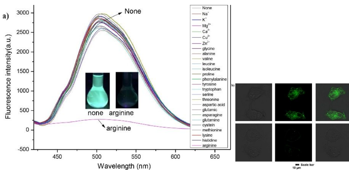
Fig. 21: a) Fluorescence spectra of probe 15 in the presence of various metal ions and amino acids THF/H 2 O system b) Fluorescence images of MCF-7 cells with probe 15 with arginine. Reproduced with permission from ref. 60. Copyright 2024 elsevier.
