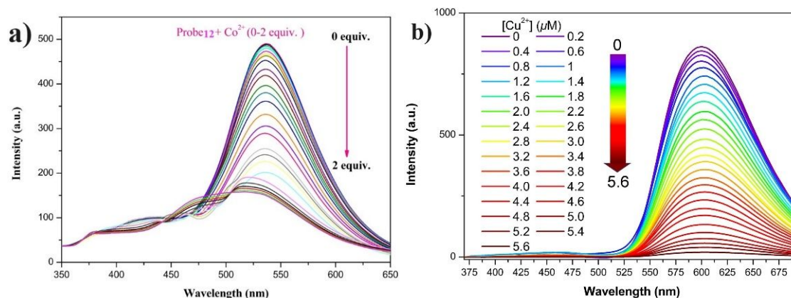
Fig. 18: a) Emission spectra of probe 12 upon increasing concentrations of Co 2+ ions in THF/H 2 O mixtures ( f_w = 60\% , pH = 7.4, \lambda_{ex} = 330 nm). b) emission spectra of probe 13 with increasing Cu 2+ ions concentration in THF/H 2 O ( f_w = 90\% , pH = 7.4, \lambda_{ex} = 350 nm). Reproduced with permission from ref. 57. Copyright 2023 springer.
