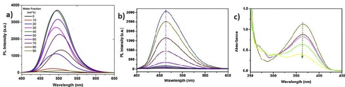
Fig. 2: a) Emission spectra of probe 1 in THF- \text{H}_2\text{O} mixtures; b) Change in the emission spectra of 1 upon increasing the concentrations of \text{Hg}^{2+} ions in THF; (c) Absorption spectra of 1 upon increasing concentrations \text{Hg}^{2+} ions in THF. Reproduced with permission from ref. 47. Copyright 2014 elsevier.
