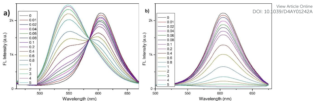
Fig. 10: a) Fluorescence spectra of probe 6 with different concentrations of Zn^{2+} in THF/ H_2O b) Fluorescence spectra of probe 6 with different concentrations of Cu^{2+} ions in THF/ H_2O . Reproduced with permission from ref. 52. Copyright 2022 elsevier.
