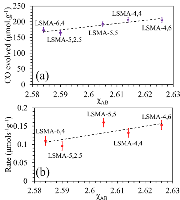
Fig. 8 Amounts of CO evolved (a) and re-oxidation rates (b) as a function of overall electronegativity of cationic components for \text{La}_x\text{Sr}_{1-x}\text{Mn}_y\text{Al}_{1-y}\text{O}_3 oxygen carriers.
