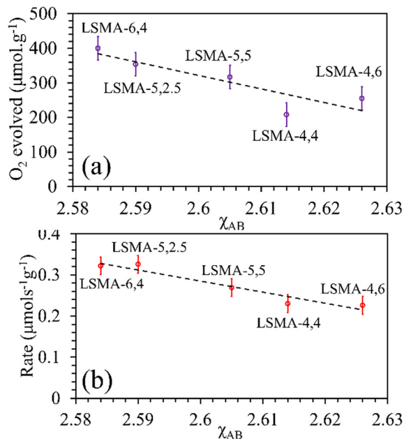
Fig. 7 Amounts of O_2 evolved (a) and reduction rates (b) as a function of overall electronegativity of cationic components for \text{La}_x\text{Sr}_{1-x}\text{Mn}_y\text{Al}_{1-y}\text{O}_3 oxygen carriers.
