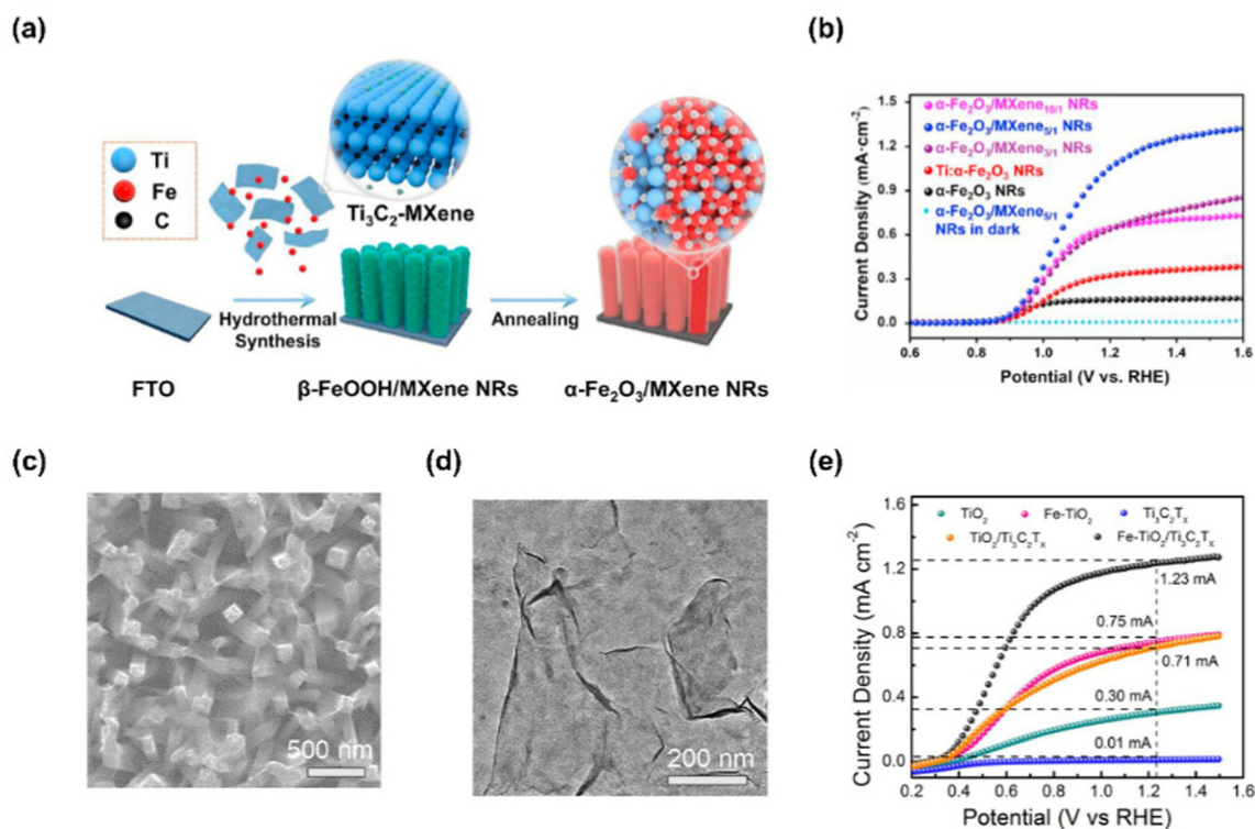
Fig. 11 (a) Schematic of fabrication process for \alpha\text{-Fe}_2\text{O}_3/\text{MXene} , NRs. (b) LSV curves \alpha\text{-Fe}_2\text{O}_3 , NRs, Ti- \alpha\text{-Fe}_2\text{O}_3 , \alpha\text{-Fe}_2\text{O}_3/\text{MXene}_{5/1} NRs, \alpha\text{-Fe}_2\text{O}_3/\text{MXene}_{10/1} NRs, and \alpha\text{-Fe}_2\text{O}_3/\text{MXene}_{1/1} NRs. Copyright 2021, Elsevier. (c) SEM image of the Fe- \text{TiO}_2/\text{Ti}_3\text{C}_2\text{T}_x . (d) TEM image of the exfoliated \text{Ti}_3\text{C}_2\text{T}_x nanosheets. (e) LSV curves of \text{TiO}_2 , \text{Ti}_3\text{C}_2\text{T}_x , \text{TiO}_2/\text{Ti}_3\text{C}_2\text{T}_x , Fe- \text{TiO}_2 (Fe: 5 mol%) and Fe- \text{TiO}_2/\text{Ti}_3\text{C}_2\text{T}_x . Copyright 2022, Elsevier.
