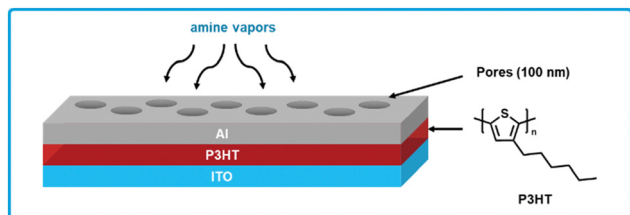
Fig. 12 P3HT based chemiresistive biogenic amine sensor. Cross-section showing the sandwich architecture with an ITO bottom electrode, P3HT active layer, and porous aluminum top electrode. Adapted with permission from L. Y. Chang, M. Y. Chuang, H. W. Zan, H. F. Meng, C. J. Lu, P. H. Yeh and J. N. Chen, ACS Sens. , 2017, 2 , 531–539. Copyright 2017 American Chemical Society. 163
