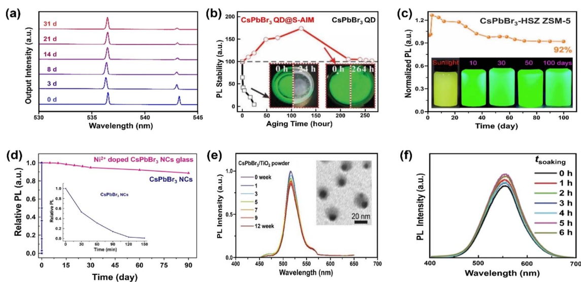
Fig. 6 Stabilizing MHPs by using inorganic materials. (a) Time-dependent normalized lasing spectra of the ALD Al 2 O 3 coated CsPbBr 3 nanoplate after being immersed in water for 1 month. Adapted from ref. 158. Copyright 2020 American Chemical Society. (b) PL intensity evolution over CsPbBr 3 QDs and CsPbBr 3 QDs@superhydrophobic aerogel inorganic matrix (S-AIM) completely immersed in water with time. Adapted from ref. 163. Copyright 2020 John Wiley and Sons. (c) PL stability of CsPbBr 3 -HSZ ZSM-5-700 composites when exposed in water and luminescent photographs of CsPbBr 3 -HSZ ZSM-5-700 composite immersed in water for various time (5 mg mL -1 ). Adapted from ref. 175. Copyright 2022 Elsevier. (d) The change in relative PL of Ni 2+ doped CsPbBr 3 NCs glass and CsPbBr 3 NCs in water (inset: enlarged the change of PL with CsPbBr 3 NCs in water). Adapted from ref. 177. Copyright 2019 Elsevier. (e) The relative PL intensity of CsPbBr 3 /TiO 2 NCs after immersing in Milli-Q water (0–12 weeks), inset shows a TEM image of CsPbBr 3 /TiO 2 NCs after immersing in Milli-Q water for 12 weeks. Adapted from ref. 181. Copyright 2017 John Wiley and Sons. (f) Normalized PL spectra of Cs 2 Sn 0.89 Te 0.11 Cl 6 versus different soaking time. Adapted from ref. 180. Copyright 2020 John Wiley and Sons.
