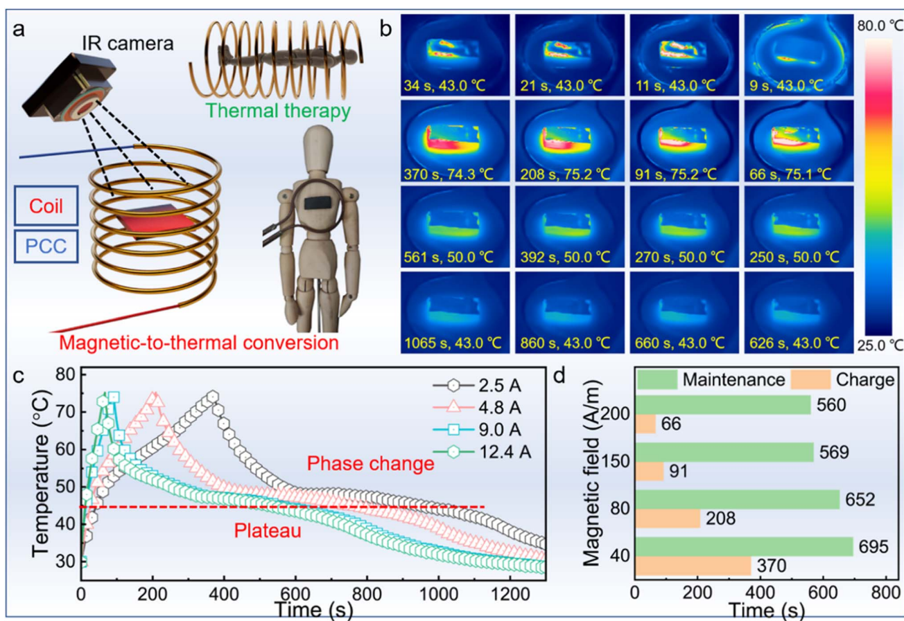
Fig. 8 (a) The illustration of magnetic-to-thermal conversion in thermal therapy application. (b) In-time images of the PCC with a current of 2.5, 4.8, 9.0, and 12.4 A. (c) Temperature curves of the PCC with a current of 2.5, 4.8, 9.0, and 12.4 A. (d) Charge and temperature maintenance performances of the PCC.
