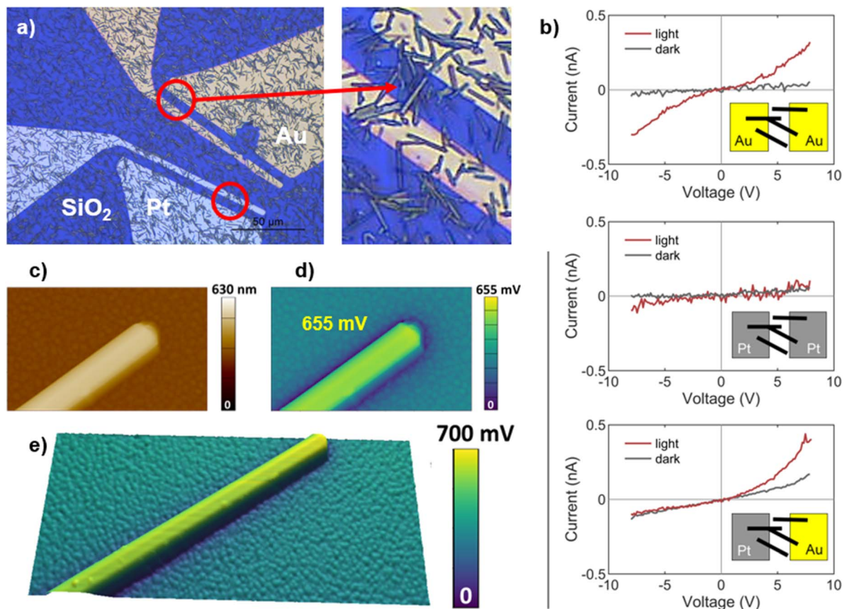
Fig. 6 (a) Optical microscope image of SbSeI crystals deposited on a Si/SiO 2 substrate with prepatterned Au and Pt contacts. (b) J – V measurements performed on a SbSeI micro-column connected to metal contacts by Schottky barrier. The following metals have been used: Au contacts, Pt contacts, Au and Pt contacts (Au as source). (c) and (d) show the topographical and surface potential map of a micro-column lying on a polycrystalline gold surface. The color scale reflects the difference of SP respect to the surrounding gold surface. (e) KPFM image – corresponds to surface potential colour map overlapped with height topology image. Height of the column is 787 nm and the SP 700 mV.
