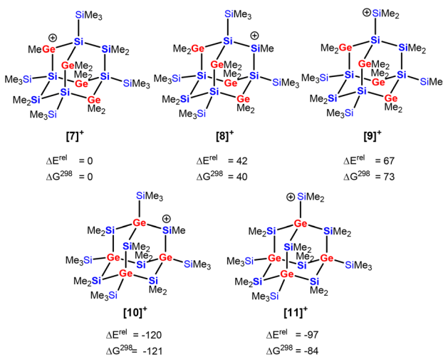
Fig. 4 Relative energies \Delta E^{\text{rel}} and free enthalpies \Delta G^{298} of \text{Si}_{10}\text{Ge}_4\text{-Me}_{23} cations derived from heteroadamantanes 3 ([7] + –[9] + ) and 4 from ([10] + , [11] + ), in kJ mol -1 , at M06-2X/6-311+G(d,p).
