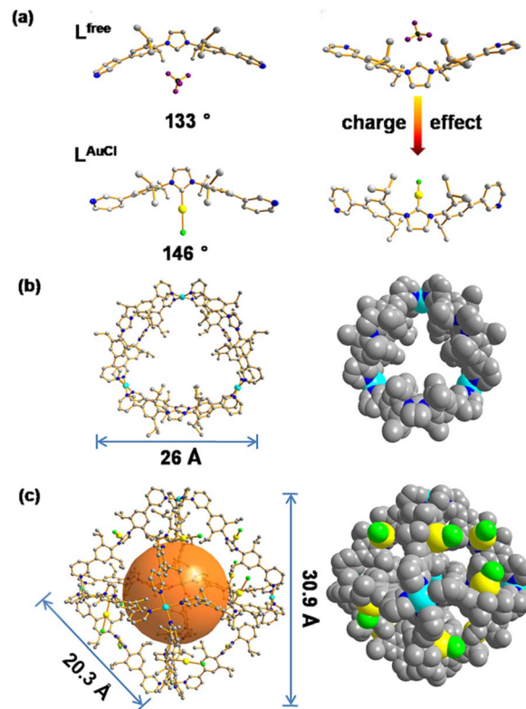
Fig. 4 (a) Single crystal X-ray structures of \text{L}^{\text{free}} and \text{L}^{\text{AuCl}} . (b) MD simulated structures of \text{Pd}_6\text{L}^{\text{free}_6} , ball-and-stick and space-filling models. (c) Single crystal X-ray structures of \text{Pd}_6\text{L}^{\text{AuCl}}_{12} , ball-and-stick model and space-filling models. Color coding: C: gray; N: dark blue; Au: yellow; Pd: light blue; Cl: bright green; B: dark green; F: violet.
