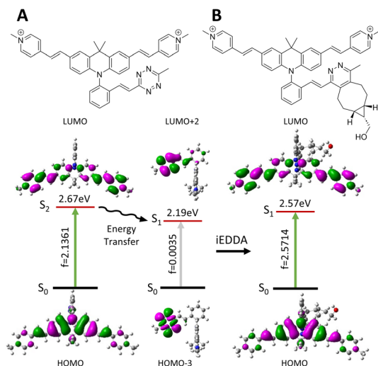
Fig. 5 Molecular structures, optimized geometries, corresponding oscillator strength ( f ) and dominating frontier molecular orbitals involved during these transitions of (A) Acridine- ovi and (B) Clicked Acridine- ovi .
