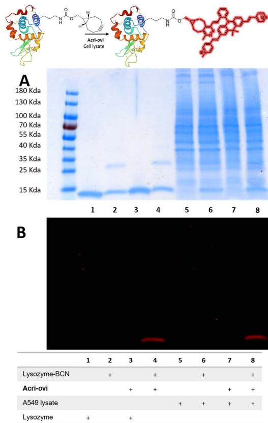
Fig. 6 Reaction of Acridine- ovi with lysozyme-BCN in the presence or absence of cell lysate. SDS-PAGE (10 \mu\text{g} per well). (A) Coomassie blue staining; (B) Fluorescence staining ( \lambda_{\text{exc}} = 496 \text{ nm} ).
