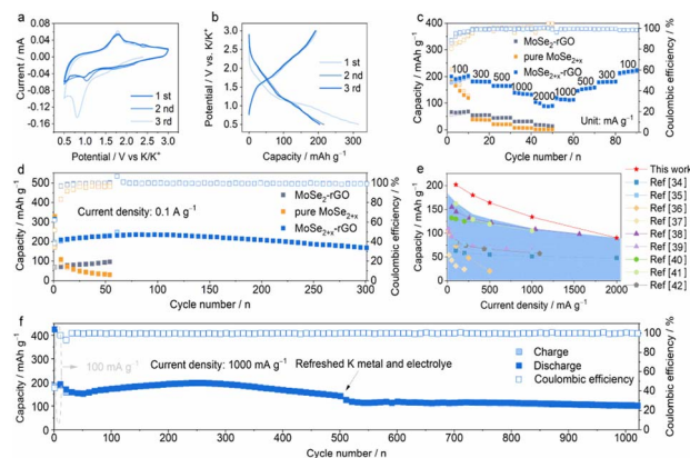
Fig. 3 Electrochemical performance of \text{MoSe}_{2+x} -rGO for potassium-ion storage. (a) CV profiles of \text{MoSe}_{2+x} -rGO for the 1st, 2nd and 3rd cycles. (b) Discharge/charge curves of \text{MoSe}_{2+x} -rGO at the 1st, 2nd and 3rd cycles. (c) Rate performance of pure \text{MoSe}_{2+x} , \text{MoSe}_{2+x} -rGO and \text{MoSe}_2 -rGO at various current densities. (d) Cycling performance of \text{MoSe}_{2+x} -rGO, pure \text{MoSe}_{2+x} and \text{MoSe}_2 -rGO at 100\text{ mA g}^{-1} . (e) Comparison of the capacity of \text{MoSe}_{2+x} -rGO with those of other cathodes at different current densities for PIBs (blue represents Prussian blue analogues/cyanoferrates, orange represents polyanionic compounds, purple represents metal oxides, green represents organic materials, and grey represents metal organic frameworks). (f) Cycling performance of \text{MoSe}_{2+x} -rGO at 1000\text{ mA g}^{-1} .
