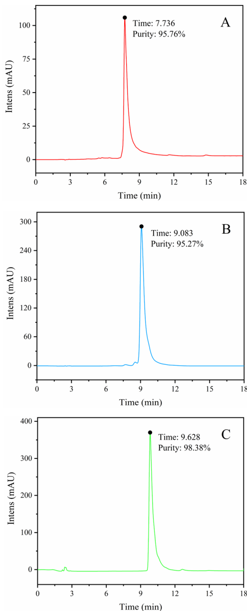
Fig. 3 HPLC spectra of W1 (myricetin-3- O -glucoside) (A), W2 (myricetin-3- O -araboside) (B), and W3 (myricitrin) (C).
