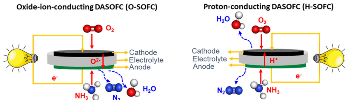
Fig. 4 Schematic representation of a direct ammonia solid oxide fuel cell based on oxide-ion-conducting (O-DASOFC) and proton-conducting (H-DASOFC) electrolytes.
