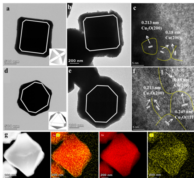
Fig. 1 Structural characterization of catalysts. The TEM images of T-Cu 2 O viewed along the (a) [100] and (d) [111] directions, and the (b and e) TEM images, (c and f) HR-TEM images, (g) HAADF-STEM and elemental mapping images (Cu species were in red, and O species were in yellow) of surface-reconstructed T-Cu 2 O samples after reduction at -1.1 V vs. RHE.
