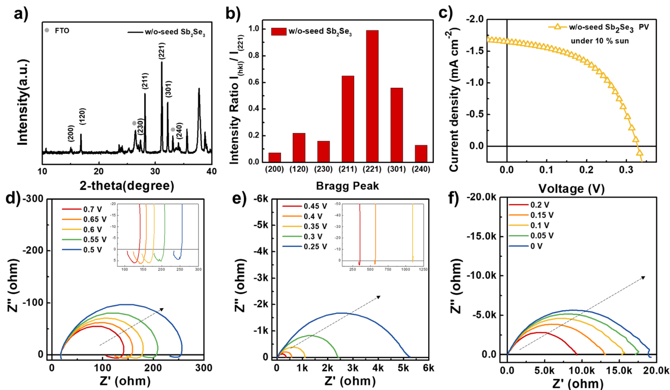
Fig. 4 (a) Diffraction patterns and (b) peak intensities ratio ( I_{(hkl)}/I_{(221)} ) of the obtained w/o-seed Sb 2 Se 3 films (c) J–V behavior exhibited by the w/o-seed Sb 2 Se 3 PV under 10% sun illumination. (d–f) Nyquist plots of the w/o-seed Sb 2 Se 3 PV at the designated applied potential.
