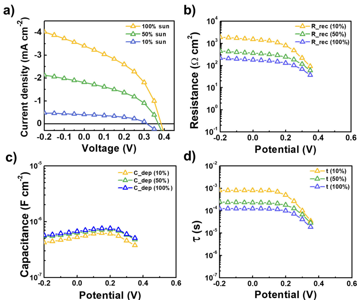
Fig. 5 (a) Steady-state photocurrent densities of the w/o-seed Sb 2 Se 3 -based PV during IS measurement under 10%, 50%, and 100% sun illumination. (b) Resistances, (c) capacitance, and (d) time constants for the charge transfer of w/o-seed Sb 2 Se 3 PV from the IS fitting procedure.
