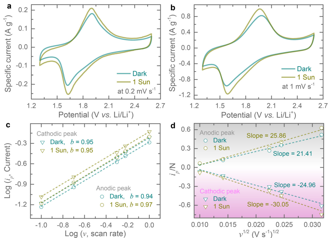
Fig. 3 Electrochemical performance of Cu-HHB electrodes both in the dark and 1 sun illuminated conditions. (a and b) CV profiles at 0.2 \text{ mV s}^{-1} and 1 \text{ mV s}^{-1} in the dark and 1 sun illumination. (c) Plots of \log(i_p) vs. \log(v) : estimation of b -values for cathodic and anodic peaks in the dark and 1 sun illumination. (d) Estimation of Li-ion diffusion constant improvements under illumination from i_p/N vs. v^{1/2} curves.
