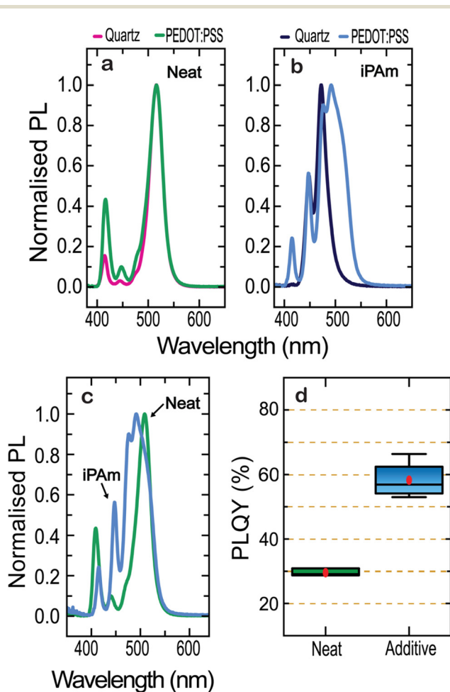
Fig. 2 Photoluminescence characteristic of \langle n \rangle = 2 thin films deposited on quartz and PEDOT of the (a) neat system (b) and the iPAm system, (c) comparison of both systems when deposited on PEDOT, and the (d) PLQYs of 12 samples of iPAm and neat thin films.
