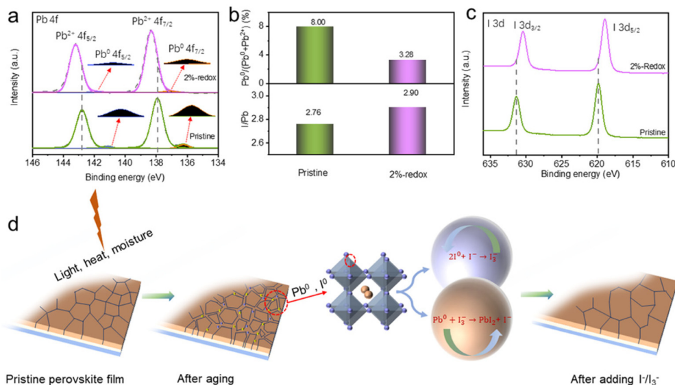
Fig. 3 (a) Pb 4f XPS spectra, (b) \text{Pb}^0/(\text{Pb}^0 + \text{Pb}^{2+}) and \text{I}/\text{Pb} ratios, (c) I 3d XPS spectra of the pristine and 2%-redox films. (d) Proposed mechanism of the \text{I}^-/\text{I}_3^- -based redox additive on passivating the \text{Pb}^0 and \text{I}^0 defects via continuous regeneration and redox reactions.
