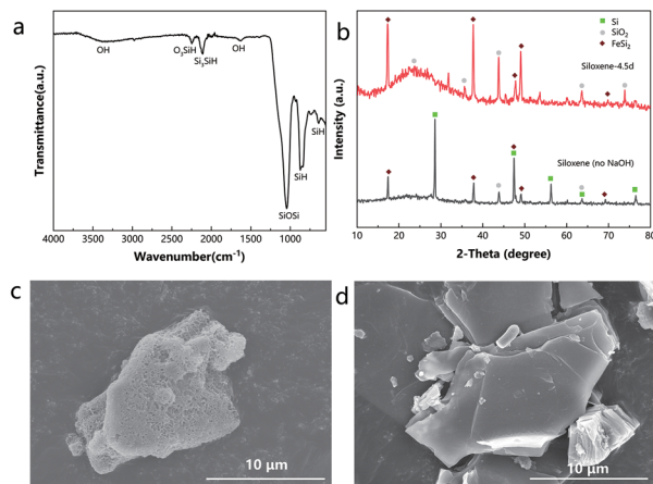
Fig. 2 (a) FTIR spectrum of siloxene-4.5d. (b) XRD patterns of siloxene (no NaOH) and siloxene-4.5d, and the peaks are labelled according to the standard \text{SiO}_2 , the standard Si, and the standard \text{FeSi}_2 . SEM images of (c) siloxene-4.5d and (d) 2DSi.
