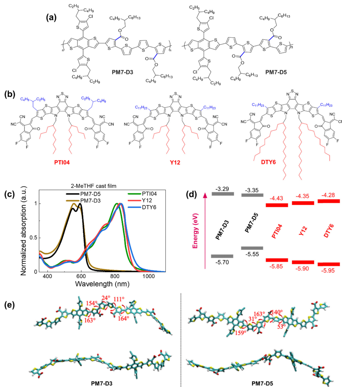
Fig. 1 Chemical structures of (a) PM7-D3 and PM7-D5 , and (b) PTI04 , Y12 , and DTY6 . (c) Normalized absorption of thin films processed from 2-MeTHF. (d) Energy level diagram of polymers donors and acceptors. (e) Top and side views of the optimized geometries (at the \omega B97X-D/6-31G(d,p) level of theory) for the symmetric dimeric models of PM7-D3 (left), and PM7-D5 (right) polymers. The dihedral angles between selected moieties are indicated in red. The long sidechains are omitted for clarity.
