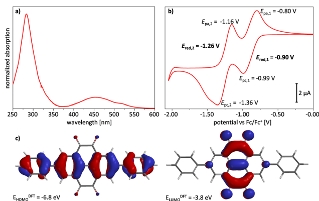
Fig. 2 (a) UV/Vis spectrum of compound 2 measured in \text{CH}_2\text{Cl}_2 at 1 \mu\text{mol L}^{-1} . (b) Cyclic voltammogram of model compound 2 ( \text{CH}_2\text{Cl}_2 , n\text{Bu}_4\text{NPF}_6 (0.1 M), measured at rt with Pt-working electrode and \text{Fc}/\text{Fc}^+ ) as internal reference, scanning velocity: 100 \text{mV s}^{-1} . (c) DFT model (B3LYP: 6-311++G**) of compound 2 (tert-butyl groups omitted).
