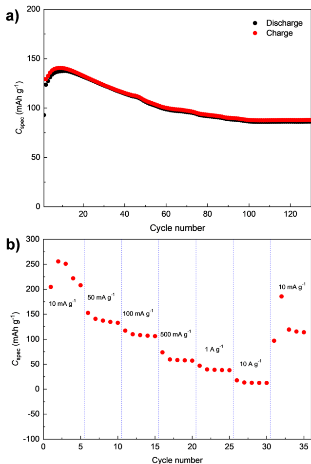
Fig. 7 Electrochemical performance of D-PTO-2a based composite electrodes within the potential range of 1.5–4 V (vs. \text{Li/Li}^+ ): (a) cycling performance at 100 \text{ mA g}^{-1} . (b) Rate performance at various current densities.
