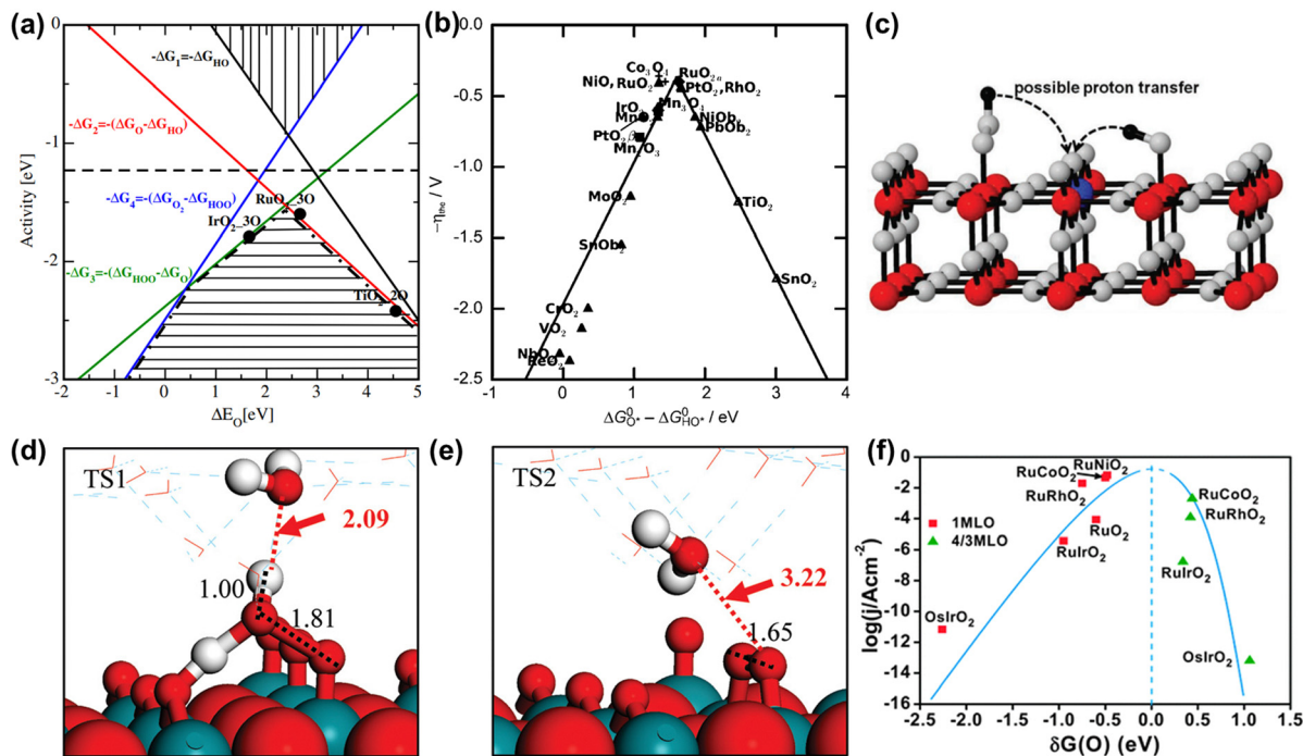
Fig. 2 (a) OER activity as a function of oxygen binding energy. (b) A volcano-type plot between OER activity and standard free energy change \Delta G_{\text{O}_2}^0 - \Delta G_{\text{H}_2\text{O}}^0 . 62 (c) Schematic illustration of the (110) surface of rutile \text{RuO}_2 modified by Ni doping. 15 (d and e) Transition state (TS) structures of water dissociation (TS1) and surface oxygen coupling (TS2) on the O-terminated phase of \text{RuO}_2(110) . 66 (f) The calculated reaction rate of OER on different oxides as a function of \delta G(\text{O}) . 67
