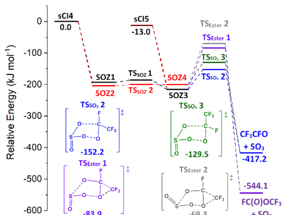
Fig. 11 The collective potential energy surface for sCIs 4 & 5 + SO 2 reactions with minima energy structures of each SO 2 fragmentation displayed. Energies are relative to the raw sCI 4 + SO 2 reactants.
