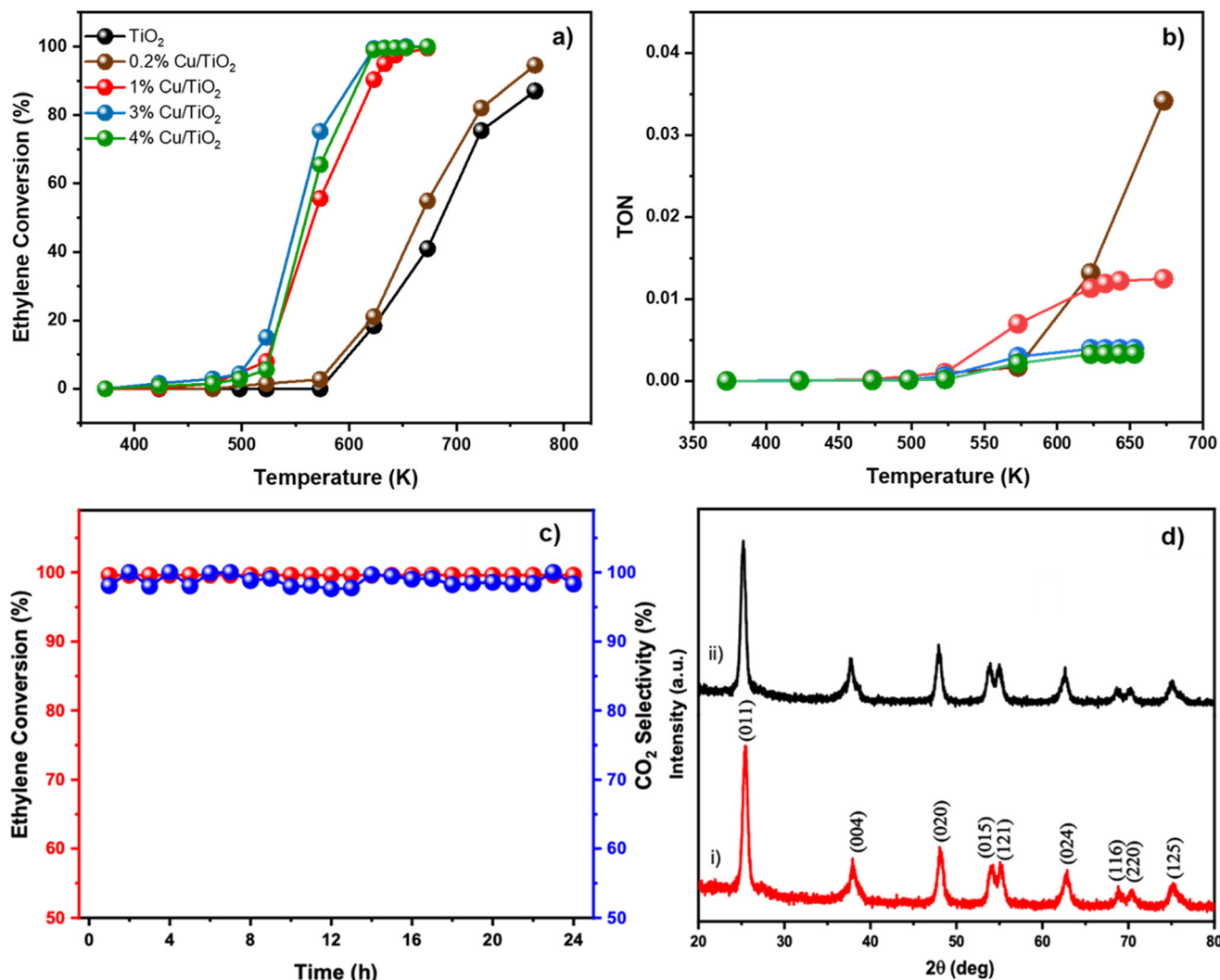
Fig. 3 a) Plots of ethylene conversion (%) against temperature (K) for \text{TiO}_2 and Cu doped \text{TiO}_2 samples (0.2%, 1%, 3% and 4%). Inset shows the colour coding for the various samples \text{TiO}_2 (black), 0.2% Cu/ \text{TiO}_2 (brown), 1% Cu/ \text{TiO}_2 (red), 3% Cu/ \text{TiO}_2 (blue) and 4% Cu/ \text{TiO}_2 (green). b) Plots of turnover number (TON) of Cu doped \text{TiO}_2 samples against temperature (K). The colour legend is same as that in a). c) Thermal stability of 1% Cu/ \text{TiO}_2 demonstrated by monitoring the conversion of ethylene at 673 K for 24 h. d) XRD patterns of 1% Cu/ \text{TiO}_2 i) before reaction and ii) after reaction for 24 h.
