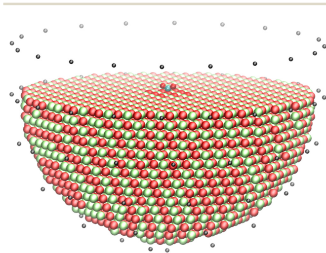
Fig. 5 ChemShell embedded cluster model of CO 2 adsorbed onto an MgO surface. Red spheres = O, green = Mg, cyan = C, black = external point charges.
