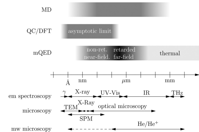
finding the relationship between the microscopic properties of systems and the resulting macroscopic effect. In other words, the microscopic properties are propagated to larger macroscopic scales. Different theoretical techniques, given in Fig. 1, have been developed to address this issue. While methods that are fully quantum (such as quantum chemistry or density functional theory) are restricted to small systems with a limited number of electrons, classical force field-based molecular dynamics (MD) simulations can treat systems consisting of a large number of molecules. An alternative to MD simulations is the quantum optical methods, in particular macroscopic quantum electrodynamics (mQED). This method considers the coupling of quantised objects via quantised fields. For this reason, it provides a higher accuracy but it does not predict single-particle responses. These properties are input parameters of this theory which provides their propagation to larger systems. Described as propagating electromagnetic waves, the relevant length scales provide different regimes: the non-retarded regime at small separations, where the finite speed of light does not matter; the retarded regime at larger lengths scales, where retardation effects of the propagating electromagnetic waves play the major role, and the thermal limit, where the interaction is driven by the thermal radiation at the specific system's temperature.
