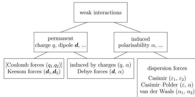
which cannot be defined by giving a particular energy threshold under which the interactions are weak and above which they are strong. In Fig. 2, a systematic scheme is presented covering the range of weak interactions based on the type of the interacting constituents in line with the traditional chemical view 16 apart from the further distinction of induced forces concerning macroscopic (bulk) responses, such as the dielectric function \epsilon . Traditionally, one restricts the dispersion forces to be induced by microscopic polarisable objects leading to the van der Waals (vdW) force. For this reason, one often denominates this class by vdW forces and includes the interactions with dielectric bodies. Nowadays, several researchers denote the entire field of weak interactions by vdW interaction, especially in chemistry and colloidal science. From the quantum-optical point of view, this makes sense by applying the electrostatic limit to the dispersive interactions. 17 In contrast, in soft-matter physics, the traditional distinction is strictly considered, and the asymptotic transitions from induced to static interactions are neglected. An overview of the denominations within the different communities is presented in Table 2. In quantum chemistry, the binding between two particles is typically considered, which leads to the phrase “non-covalent” for weak interactions. Concerning non-covalent bonding, ionic and hydrogen bonds belong to the weak interactions, see Fig. 2, as well, but will not be considered explicitly within this review.
