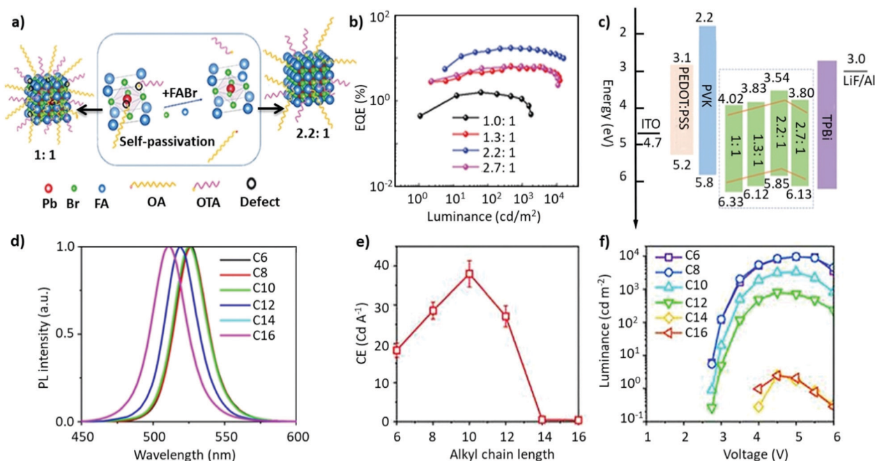
Fig. 11 (a) Reaction illustrating the self-passivation of excess FABr. (b) EQE–luminance curves of PeLEDs based on \text{FAPbBr}_3 NCs with varying molar ratios of \text{FABr}/\text{PbBr}_2 . (c) Energy-band diagram of \text{FAPbBr}_3 NCs with varying molar ratios of \text{FABr}/\text{PbBr}_2 . (d) PL emission spectra of \text{FAPbBr}_3 NCs synthesized using various chain lengths of alkylamine ligands, (e) current efficiency as a function of the alkyl chain length, and (f) luminance–voltage curves for PeLEDs with different chain lengths (from C6–C16). Panels (a–c) adapted from ref. 125. Copyright 2020 WILEY-VCH Verlag GmbH & Co. KGaA, Weinheim. Panels (d–f) reproduced with permission from ref. 193. Copyright 2019 American Chemical Society.
