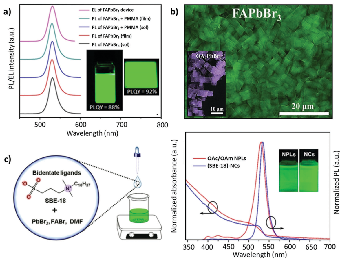
Fig. 8 (a) PL spectra for the colloidal 2D \text{FAPbBr}_3 perovskite and its composite with PMMA, where the inset depicts the 2D \text{FAPbBr}_3 perovskite colloidal solution (left) and spin-coated thin film (right) under UV excitation in toluene solution and thin films. (b) SEM image of \text{FAPbBr}_3 NPLs, where the inset depicts the SEM image of \text{OA}_2\text{PbBr}_4 . (c) Schematic illustration of the synthesis process of \text{FAPbBr}_3 NCs (left) and the PL absorption and emission spectra of (SBE-18)-capped \text{FAPbBr}_3 NCs and \text{OAc/OAm} -capped \text{FAPbBr}_3 NPLs (right), with insets showing their colloidal solutions under 365 nm UV light. Panel (a) adapted from ref. 159. Copyright 2017 American Chemical Society. Panel (b) adapted from ref. 161. Copyright 2018 WILEY-VCH Verlag GmbH & Co. KGaA, Weinheim. Panel (c) reproduced with permission from ref. 162. Copyright 2019 American Chemical Society.
