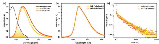
Fig. 3 Photophysical properties of 8 wt% [Ir(dpq) 2 bpy][B(5FPh) 4 ]-doped films in IAQ-PhCz and IAQ-CzCz. (a) FET evaluation between phosphor and IAQ derivatives, (b) PL spectra of doped films, and (c) PL transient decay curves measured at 640 nm.
