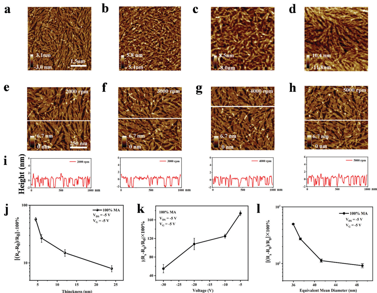
Fig. 2 (a–d) AFM images of thin films at various concentrations (0.7, 1, 3, and 5 \text{mg mL}^{-1} ) by the off-center at a rotating speed of 5000 rpm. (e–h) AFM images of LDPN films prepared by various off-center spin-coating speeds at a solution concentration of 0.7 \text{mg mL}^{-1} . (i) The corresponding height profiles along the indicated lines in (e–h). (j) The sensitivity of the resistance response against the film thickness. (k) The resistance response as a function of equivalent mean diameters. (l) The relationship between the resistance response and operation voltage.
