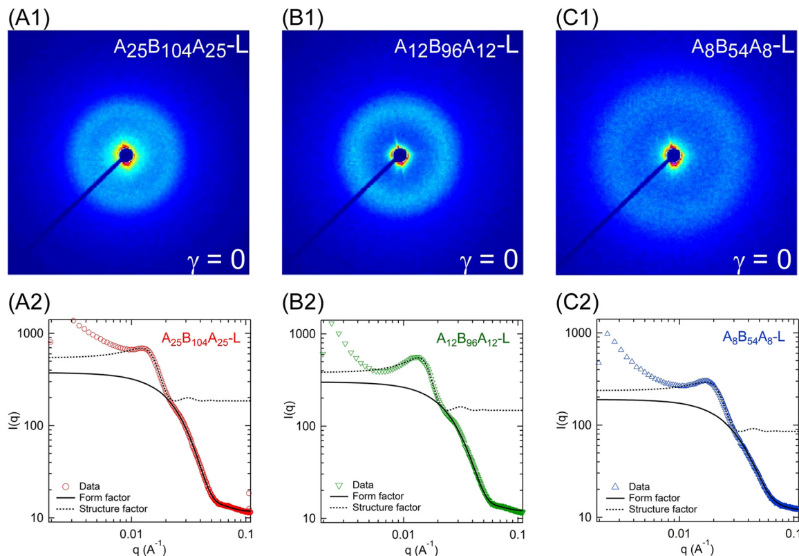
Fig. 7 2D scattering pattern for (A1) A_{25}B_{104}A_{25} -L, (B1) A_{12}B_{96}A_{12} -L, and (C1) A_8B_{54}A_8 -L at room temperature without any applied strain. The corresponding I(q) - q data and their fitting with polydispersed spheres form factor and hard-sphere structure factor are shown in A2–C2.
