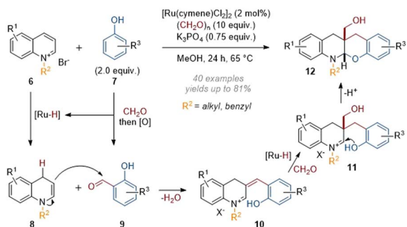
Scheme 4 Catalytic reductive tandem functionalisation of quinolinium salts with phenols and formaldehyde. 9
