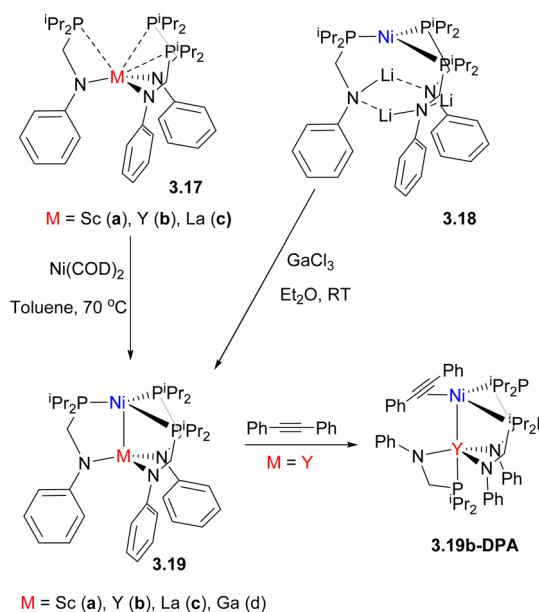
Scheme 21 The formation of Ni–RE bimetallic complexes and the formation of a structurally characterized Ni/Y–alkyne adduct enabled by ligand hemilability.
