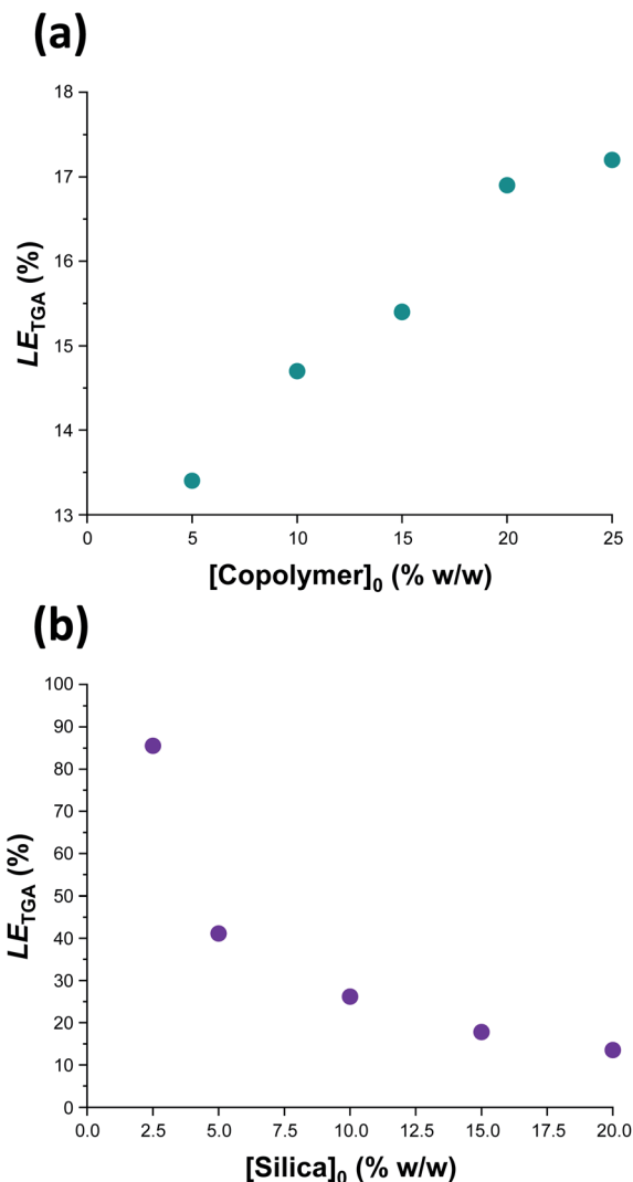
Fig. 6 Vesicle loading efficiency, LE_{TGA} , as determined by thermogravimetric analysis for: (a) a series of silica-loaded PDMAC 49 -P(HBA-stat-DAAM) 302 vesicles prepared at various copolymer concentrations using a constant silica nanoparticle concentration of 20% w/w; (b) a series of PDMAC 49 -P(HBA-stat-DAAM) 302 vesicles prepared at various silica nanoparticle concentrations using a constant copolymer concentration of 10% w/w. See Section 2.1 of the ESI† for further details of the LE_{TGA} calculation.
