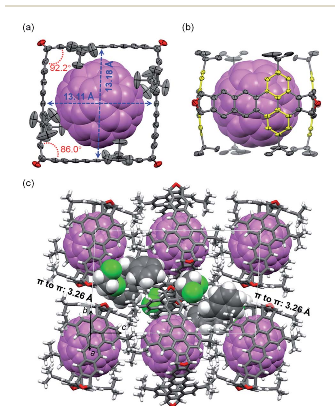
Fig. 6 Crystal structure of C_{60} \subset \mathbf{3} \cdot 2(C_2H_4Cl_2) \cdot 2(C_6H_5CH_3) : (a) top view of C_{60} \subset \mathbf{3} ; (b) side view of C_{60} \subset \mathbf{3} ; (c) molecular packing in a unit cell. C_{60} is shown in violet with a space-filling model; in panels a and b, carbon and oxygen atoms in 3 are shown as ellipsoids at the 50% probability level, and hydrogen atoms are removed for clarity; in panel c, molecules of 3 are shown with stick models, and co-crystallized solvent molecules are shown with space-filling models.
